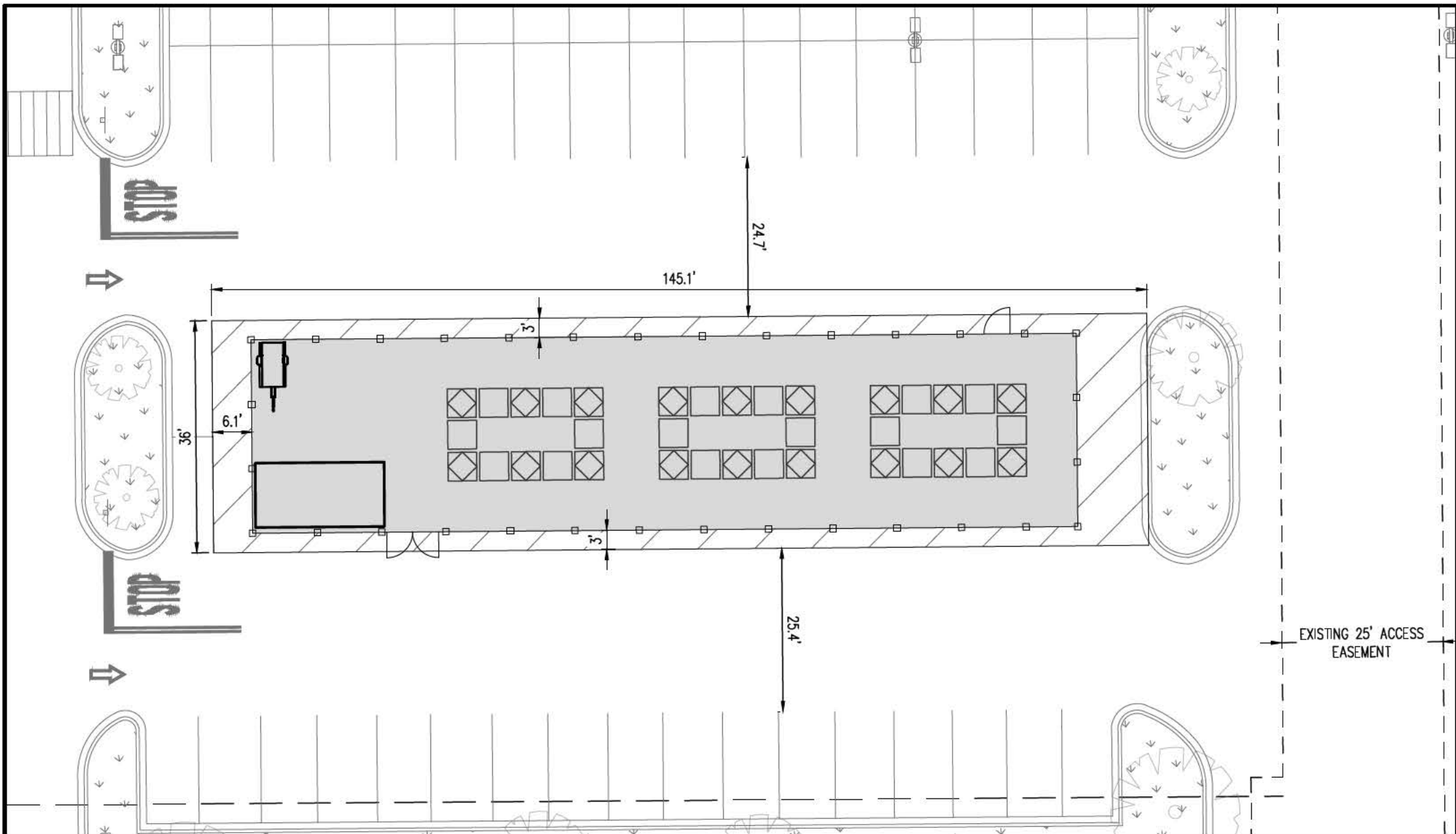
HORIZONTAL DIMENSION PLAN
