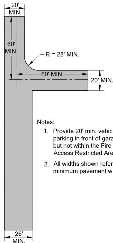
FIGURE 3 Flag Lot Turn-Around Dimensions
